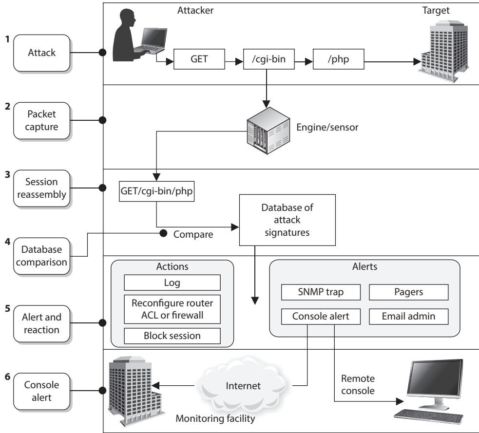
Figure 5-24 The basic architecture of a NIDS
