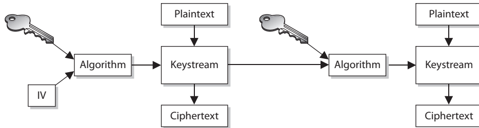
Figure 3-41 A block cipher working in OFB mode
