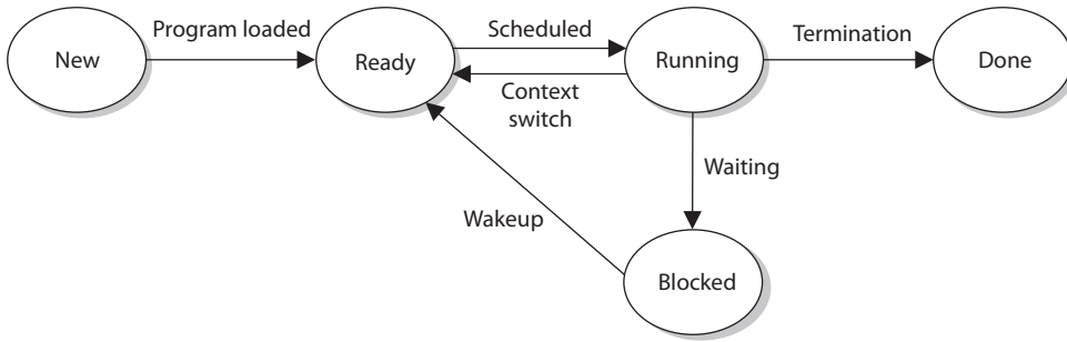
Figure 3-11 Processes enter and exit different states.
