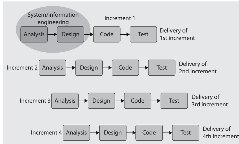
Figure 8-9 Incremental development model
