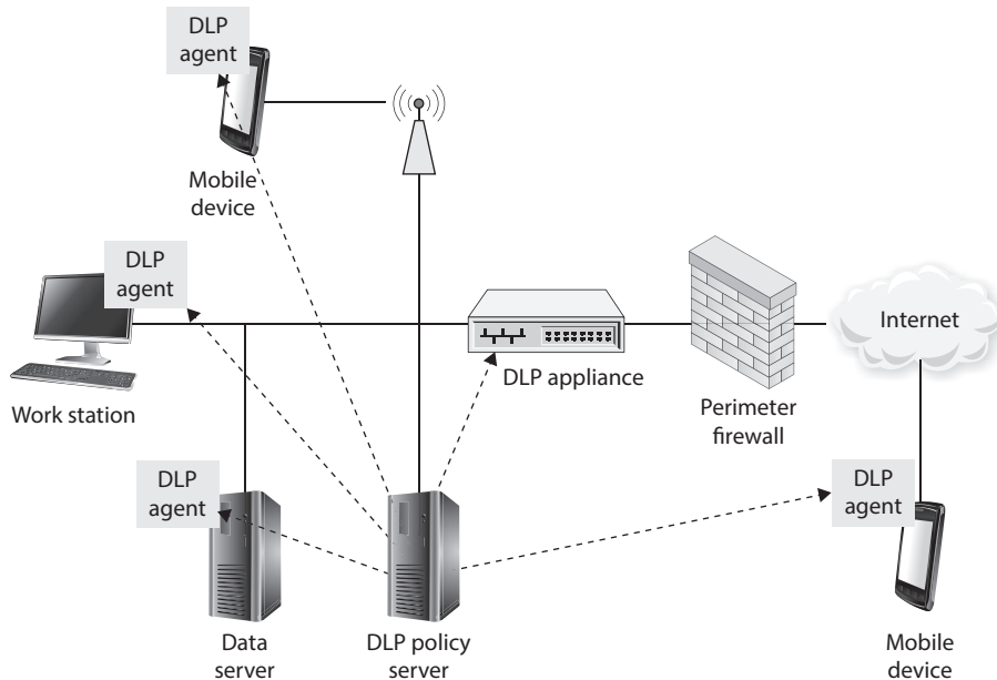
Figure 2-9 Hybrid NDLP/EDLP
