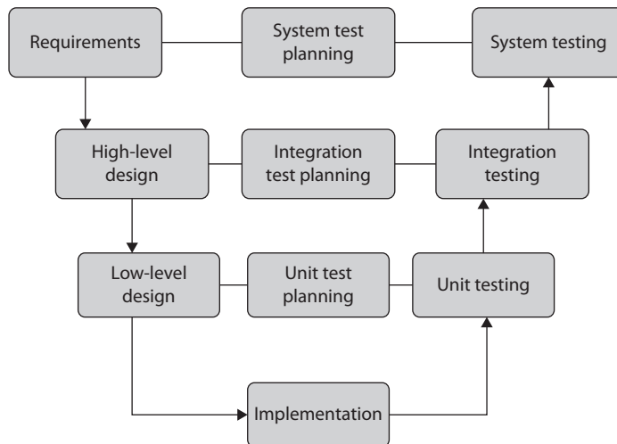
Figure 8-8 V-shaped model
