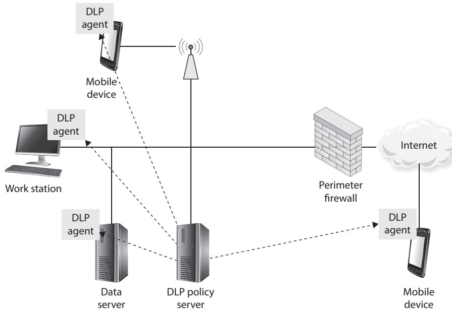
Figure 2-8 Endpoint DLP
