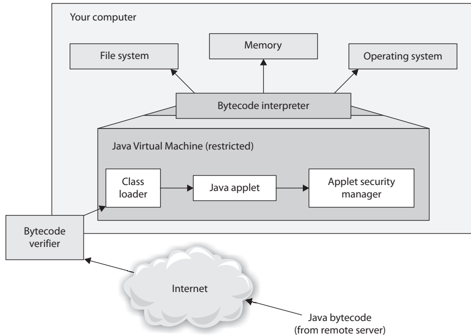
Figure 8-29 Java's security model
